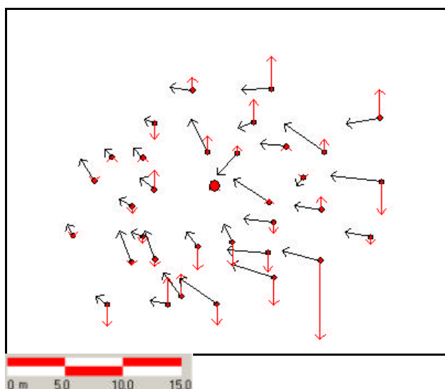
Figure 12. Horizontal and Vertical Errors with 1 GCP in the Center.
