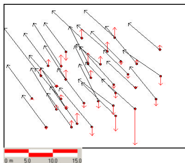
Figure 8. Horizontal and Vertical Errors without GCPs
