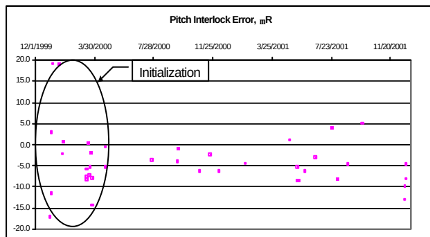
Figure 5. Time series of pitch interlock errors.
