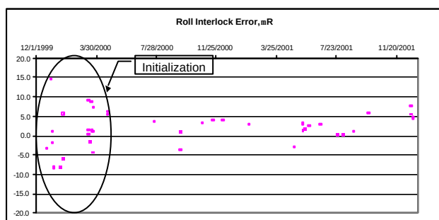
Figure 4. Time series of roll interlock errors.
