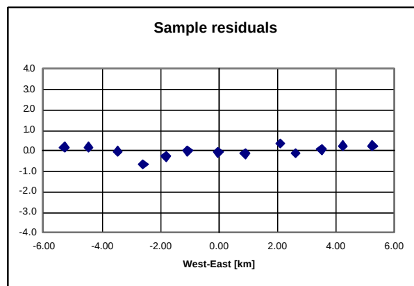
Figure 2. Post-FAM-calibration residual errors over the Southern test range.
