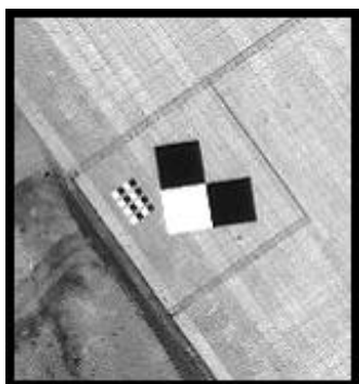
Figure 3. Space Imaging MTF Target
