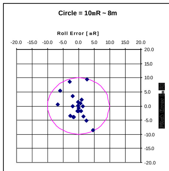
Figure 6. Post-interlock-calibration error distribution.
