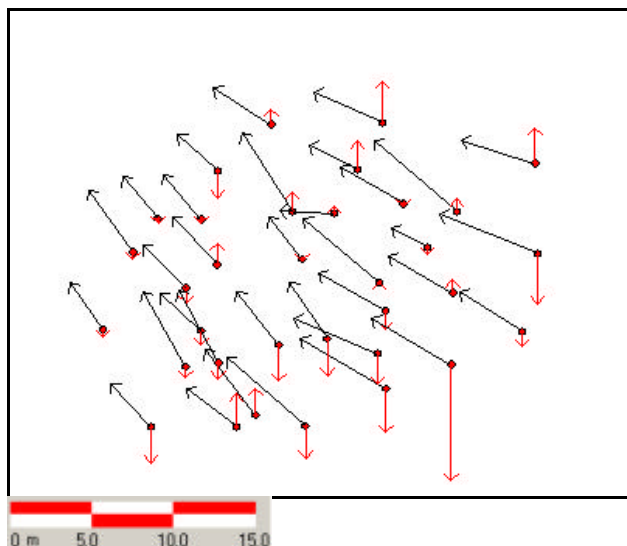
Figure 11. Horizontal and Vertical Errors without GCPs
