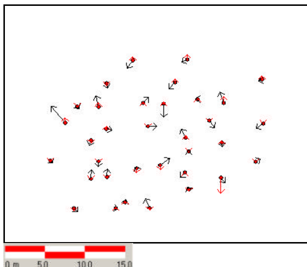
Figure 10. Horizontal and Vertical Errors with All GCPs
