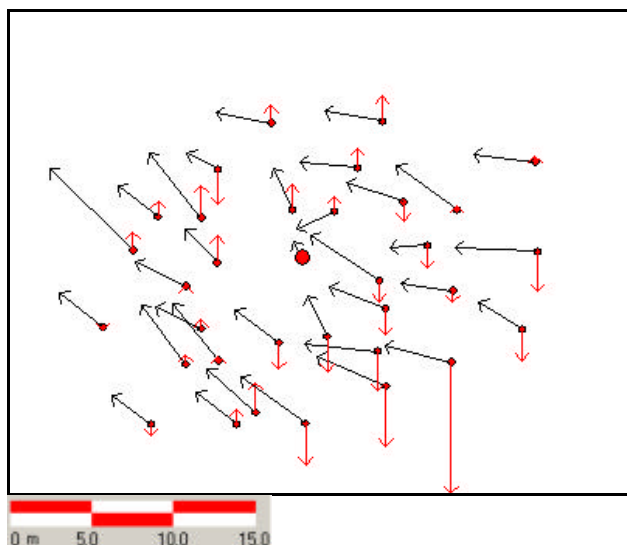
Figure 9. Horizontal and Vertical Errors with 1 GCP in the Center.
